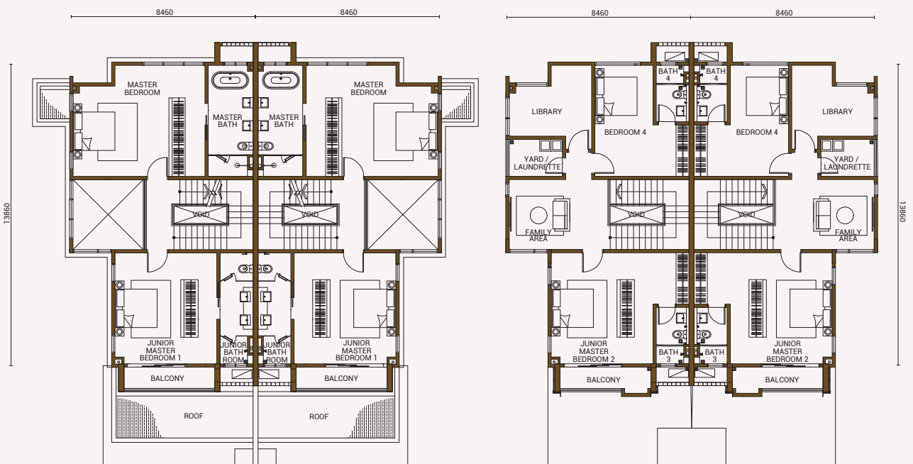
First Floor
