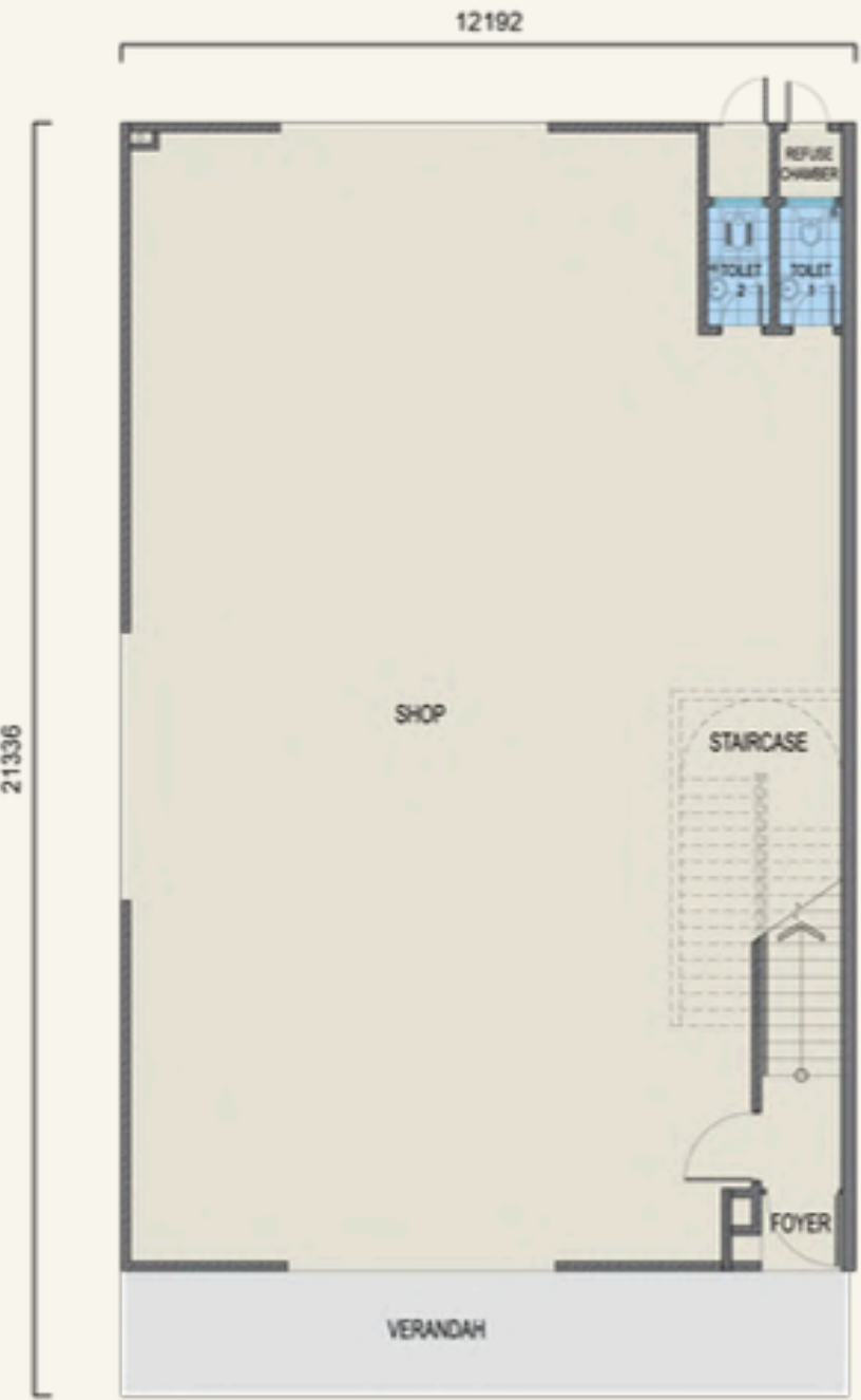
Type SE1 Ground Floor
