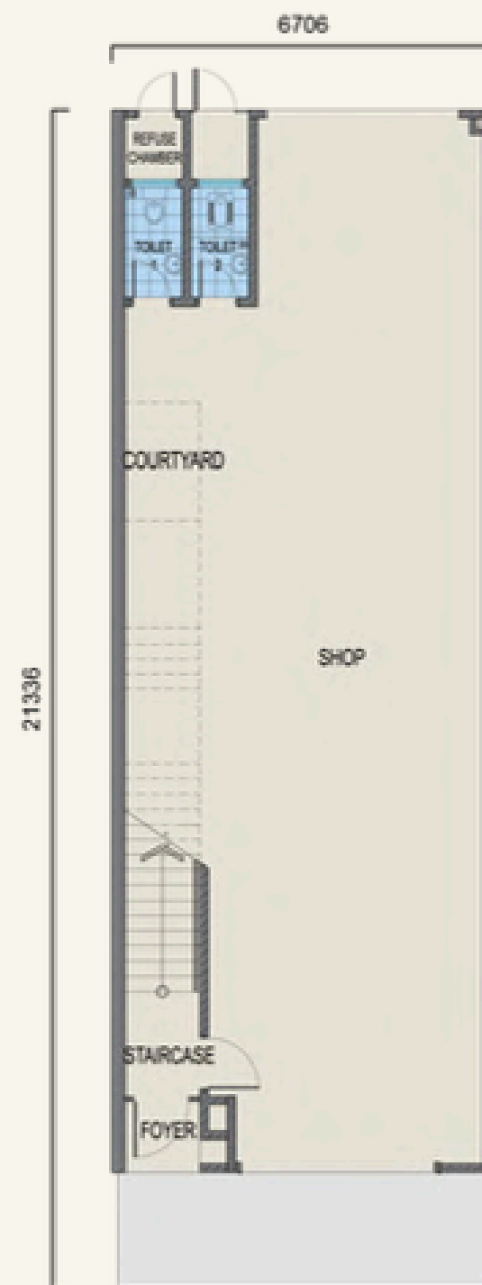
Type INC-2 Ground Floor
