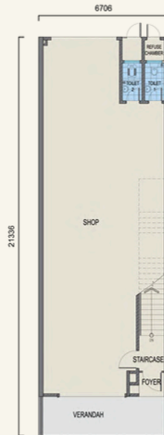
Type IN-1L Ground Floor
