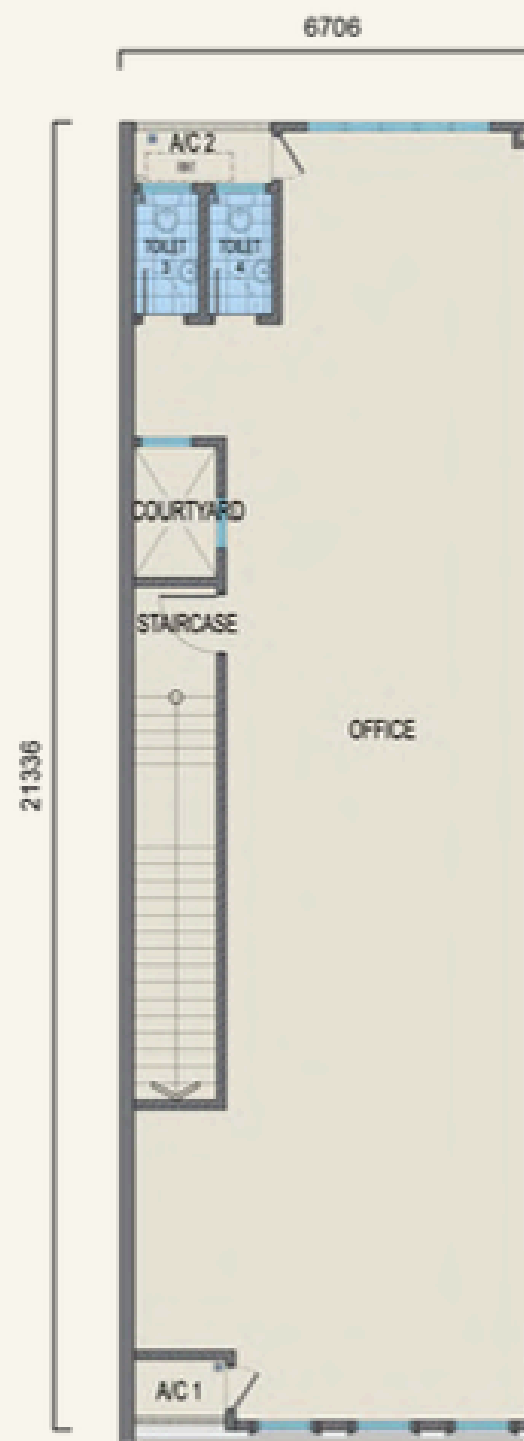
Type INC-2 First Floor
