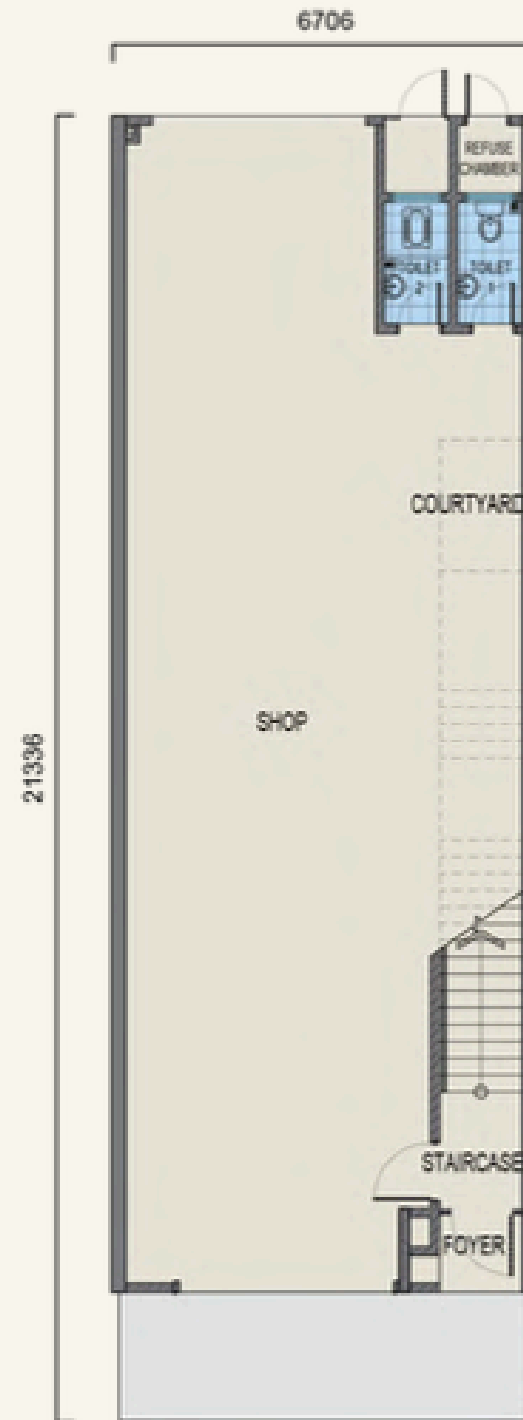
Type INC-1 Ground Floor
