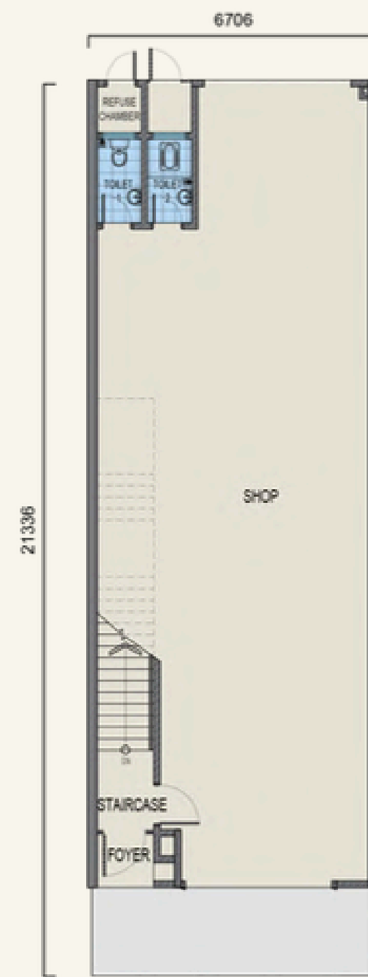
Type IN-2L Ground Floor
