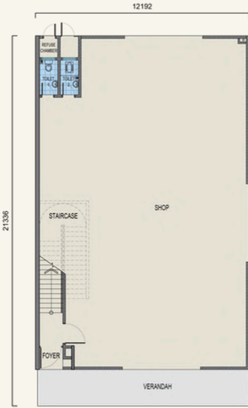
Type SE2 Ground Floor
