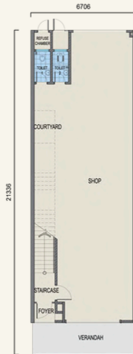
Type INC-2L Ground Floor
