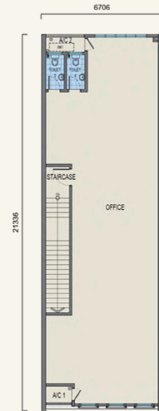
Type IN-2 First Floor
