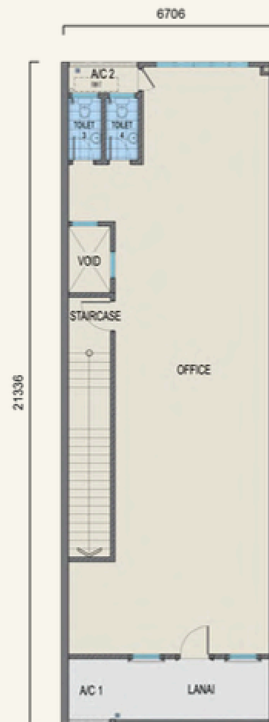
Type INC-2L First Floor
