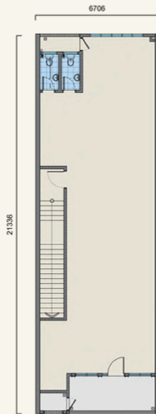
Type IN-2L First Floor
